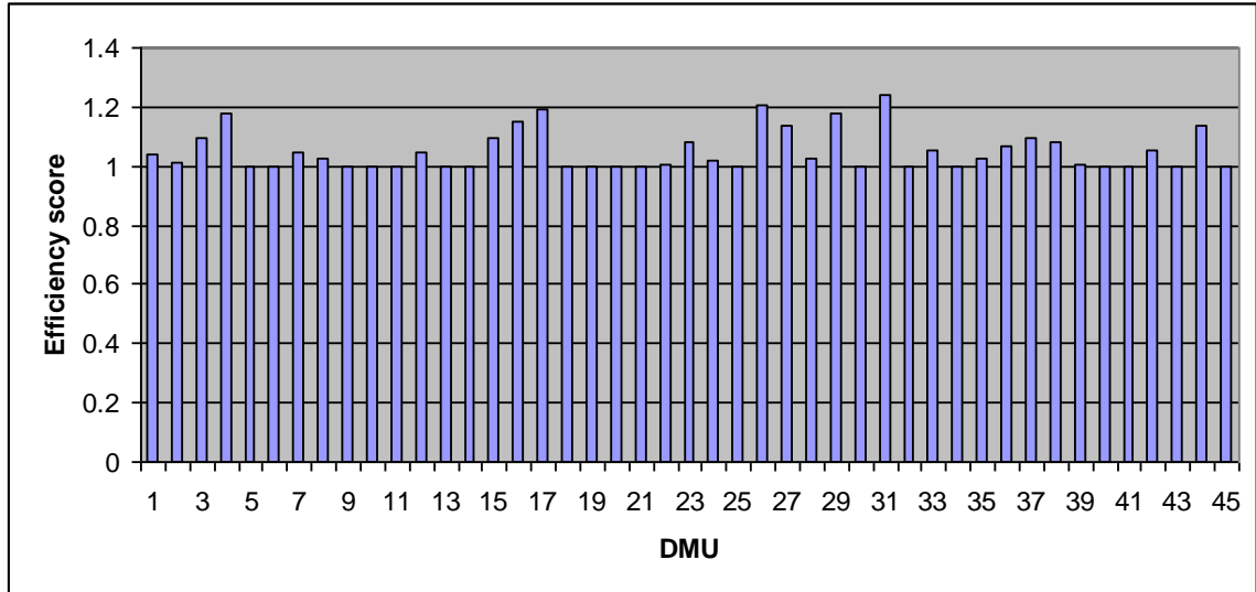
Figure 2. Estimated efficiency scores of Model II across DMUs
