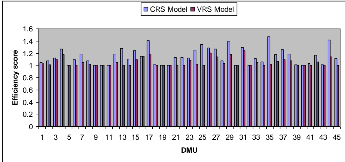
Figure 3. Efficiency scores of CRS model and VRS model
