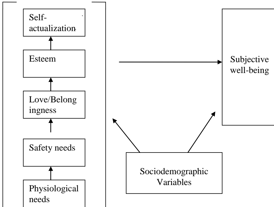
Figure 2 Conceptual framework
