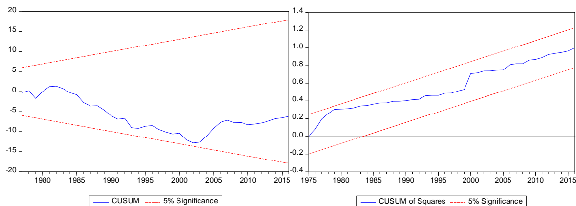
Figure 2. Plots of CUSUM and CUSUMSQ Tests (Model 4)
