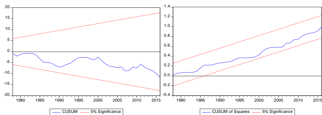
Figure 1. Plots of CUSUM and CUSUMSQ Tests (Model 3)
